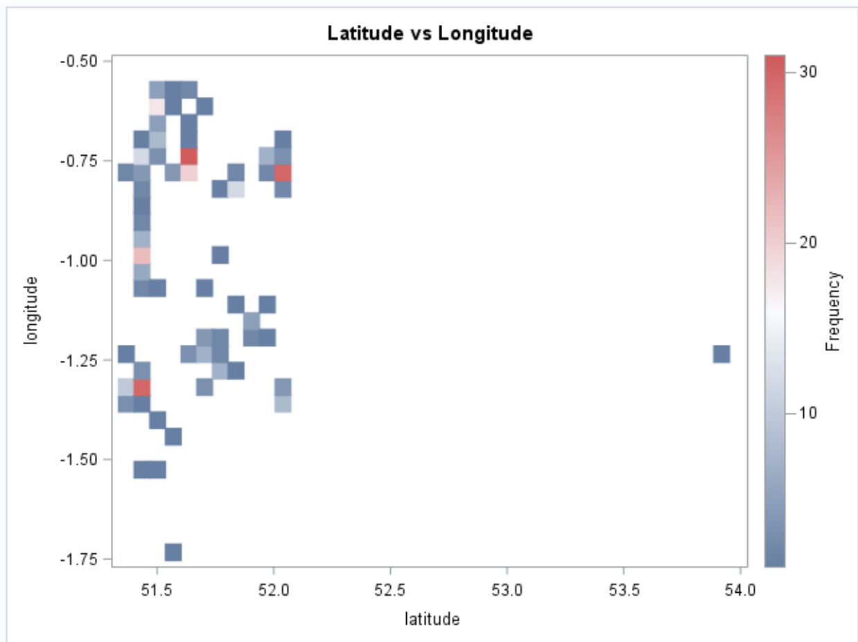
Output 11. Using the SGPLOT procedure within Jupyter Notebook to produce a heat map
